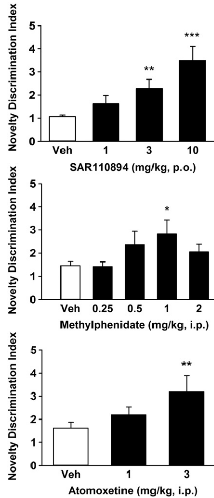
Fig. 10. Effects of SAR110894, atomoxetine and methylphenidate on spontaneous selective attention disruption in adult rats. Bars represent the mean (+S.E.M.) novelty discrimination index. Post hoc analyses (Dunnett's test) following a 2-way ANOVA: * P < 0.05 , ** P < 0.01 , *** P < 0.001 versus vehicle-treated rats. N = 10 rats per group.
