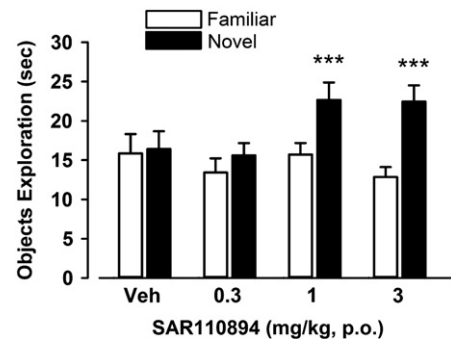
Fig. 5. Effects of SAR110894 on long-term visual episodic memory in the ORT in rats. Each bar represents the average of objects exploration time (seconds; means \pm S.E.M.) of the novel object (black columns) and of the familiar object (open columns). The interval between the acquisition and the recall session was 24 h. *** P<0.001 novel versus familiar object for each treatment group. N = 8 to 10 rats per group.
