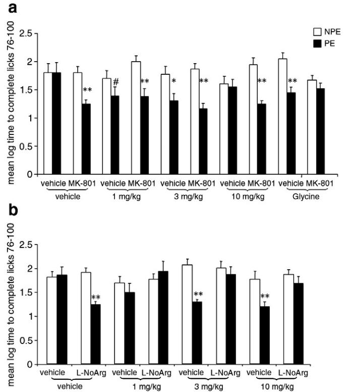
Fig. 8. Effects of SAR110894 on (a) MK-801- or (b) L-NoArg-induced persistent LI. Means and standard errors of the log times to complete licks 76–100 (after tone onset) of the pre-exposed (PE) and non-pre-exposed (NPE) rats treated with MK-801, L-NoArg or vehicle, injected with SAR110894 at doses of 1, 3 and 10 mg/kg, glycine at 0.8 g/kg or vehicle. Forty pre-exposures and 5 conditioning trials were used. SAR110894 was administered i.p. in the pre-exposure and conditioning phases. Asterisks indicate a significant difference between the PE and NPE groups, namely, presence of LI. # P = 0.07 , * P < 0.05 and ** P < 0.01 . N = 11 to 12 rats per group.
