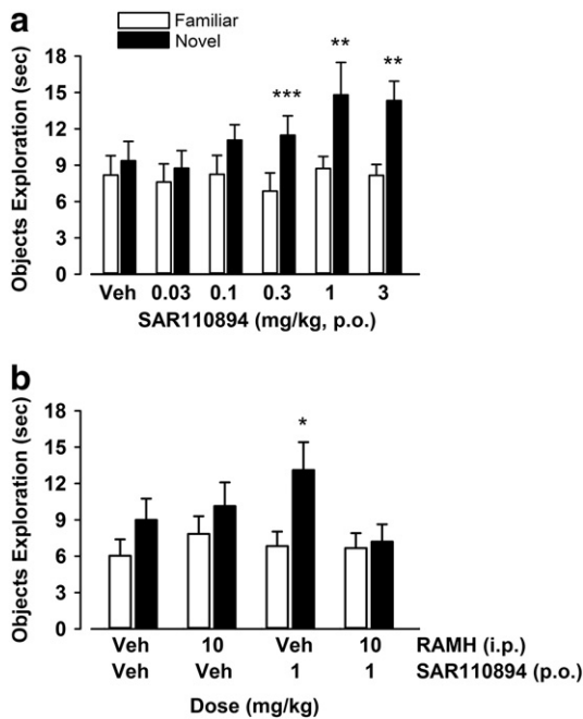
Fig. 4. a) Acute treatment with SAR110894 on long-term visual episodic memory in the ORT in mice. Each bar represents the average exploration time (seconds; means \pm S.E.M.) of the novel (black columns) and the familiar object (open columns). The interval between the acquisition and the recall session was 48 h. *** P<0.001 , ** P<0.05 novel versus familiar object for each treatment group. N = 10 to 21 mice per group. b) Antagonism by RAMH of the effects of SAR110894 on long-term episodic memory in the ORT in mice. * P<0.05 novel versus familiar object for each “RAMH” \times “Treatment” group. N = 10 to 12 mice per group.
