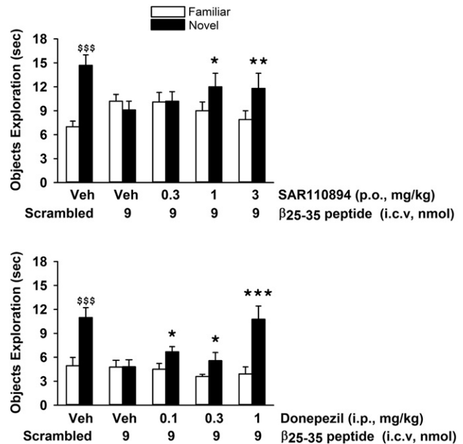
Fig. 12. Effects of SAR110894 and donepezil on \beta_{25-35} -induced visual episodic memory in mice. Data represent exploration time (mean + S.E.M.) of the novel (black columns) and familiar (open columns) object, respectively. $$$ P < 0.001 ; comparison novel versus familiar object for each treatment groups; Winer analysis following 2-way ANOVA (with "Vehicle + \beta_{25-35} " and "Vehicle + saline" groups) with repeated measurements on object. * P < 0.05 , ** P < 0.01 , *** P < 0.001 ; comparison novel versus familiar object for each treatment group; Winer analysis following 2-way ANOVA (with "Vehicle + \beta_{25-35} " and "SAR110894 or donepezil + \beta_{25-35} " groups) with repeated measurements on object. N = 5 – 8 per group.
