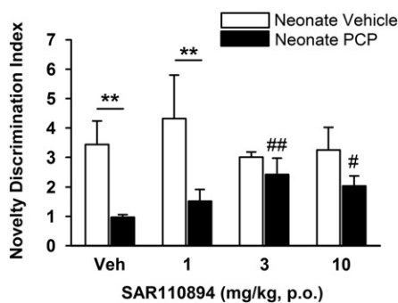
Fig. 9. Antagonism by SAR110894 of the impairment of novelty discrimination in adult rats treated with PCP at the neonatal stage. Each bar represents the mean (+S.E.M.) novelty discrimination index (ratio of the time spent investigating the novel juvenile divided by the time spent investigating the familiar juvenile, in seconds). Post hoc analyses following a 2-way ANOVA: ** P < 0.01 versus corresponding saline-neonates group; # P < 0.05 , ## P < 0.01 versus acute vehicle PCP-neonates group (Dunnett's test). N = 10 rats per group.
